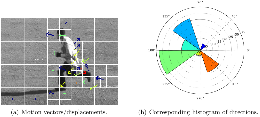
Figure 4.3: Frame with motion vectors and its corresponding histogram of directions. To avoid clutter, only one motion vector per block is shown, and not entire trajectories.
