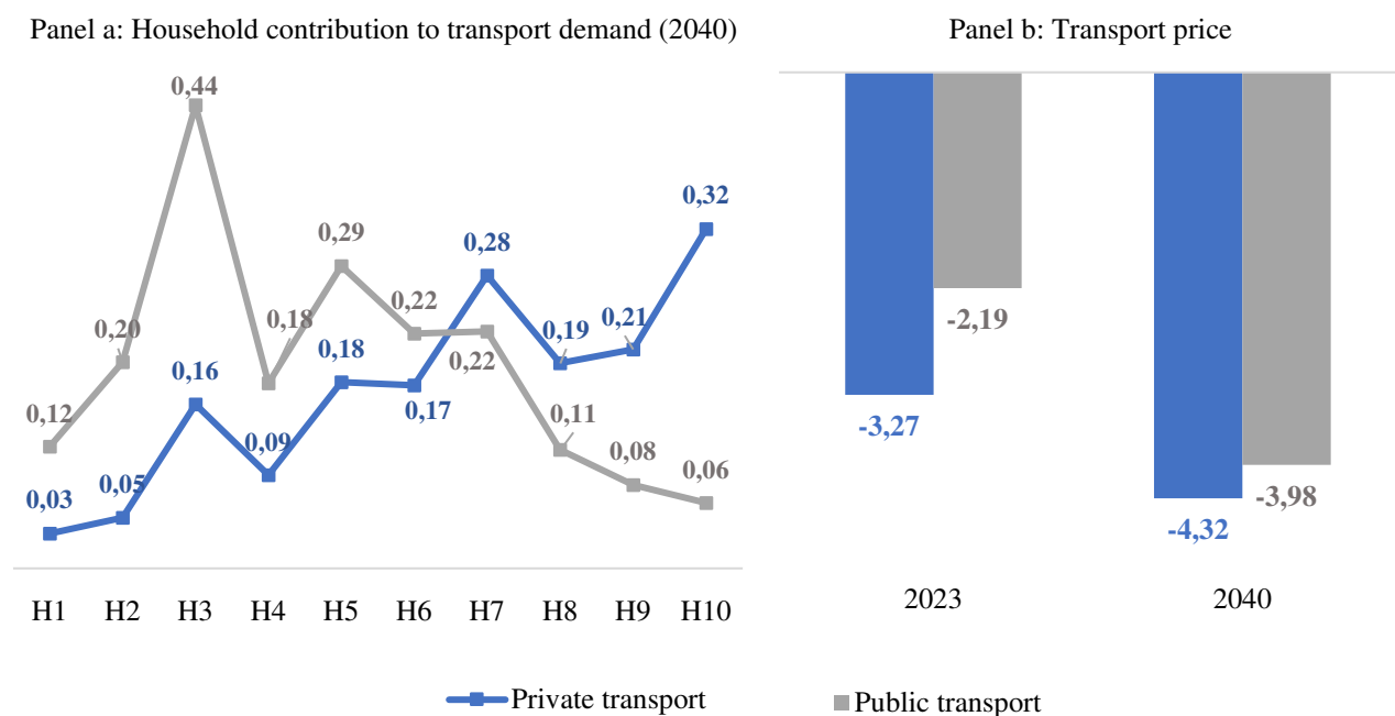
Figure 1 – Effect of policy on private and public transport
