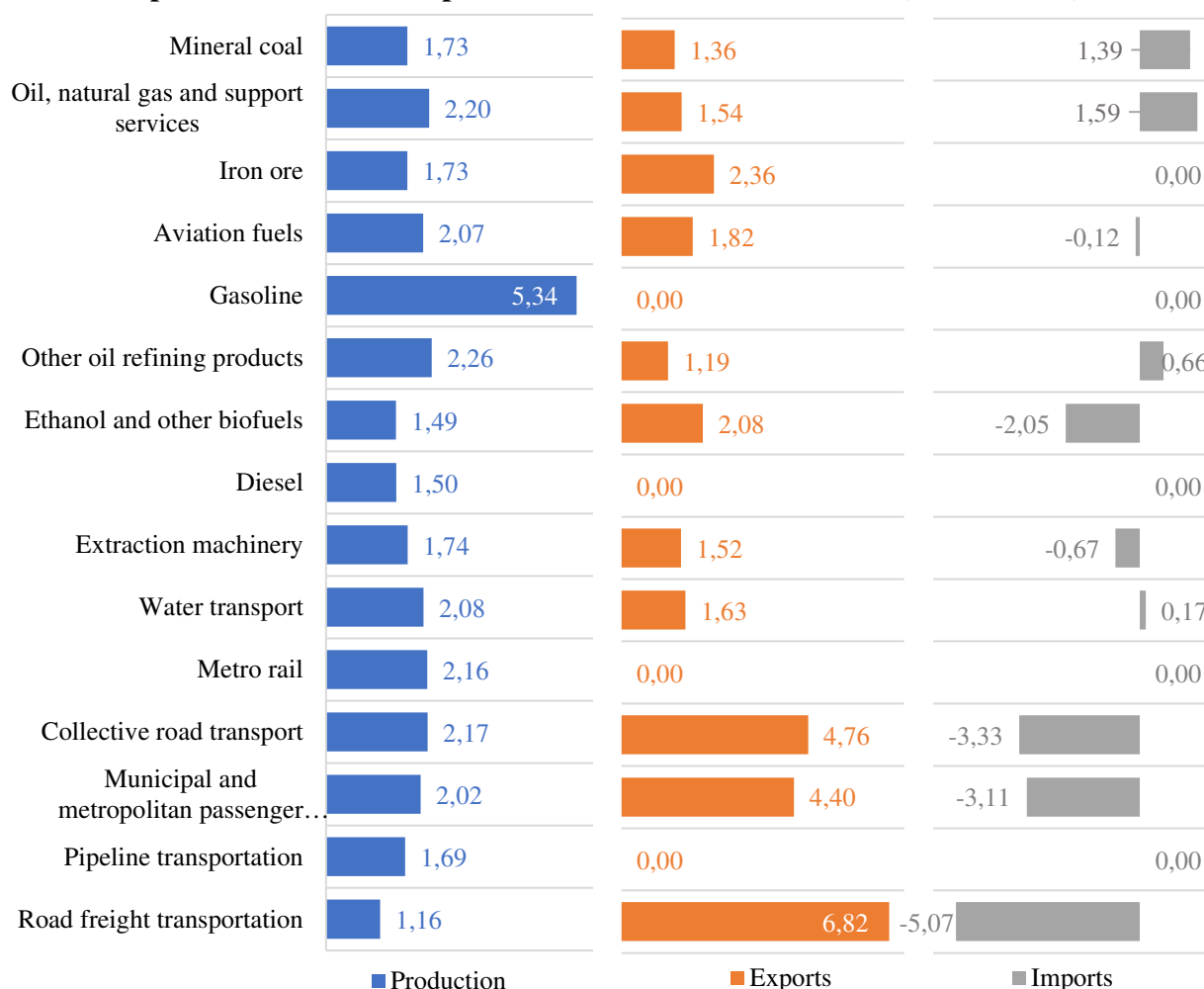
Graph 2 – Cumulative impacts on sector indicators in 2040 (BAU = 2023)
