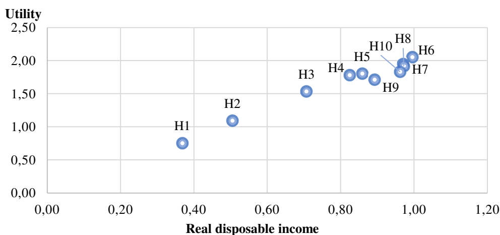
Graph 4 – Cumulative impacts on real household income and utility (2040)
