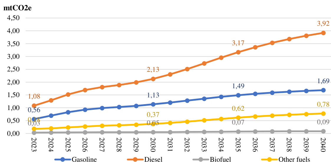
Graph 3 – Variations in GGE emissions by type of fuel burned (BAU = 2023)
